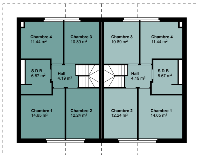
COMBLES
